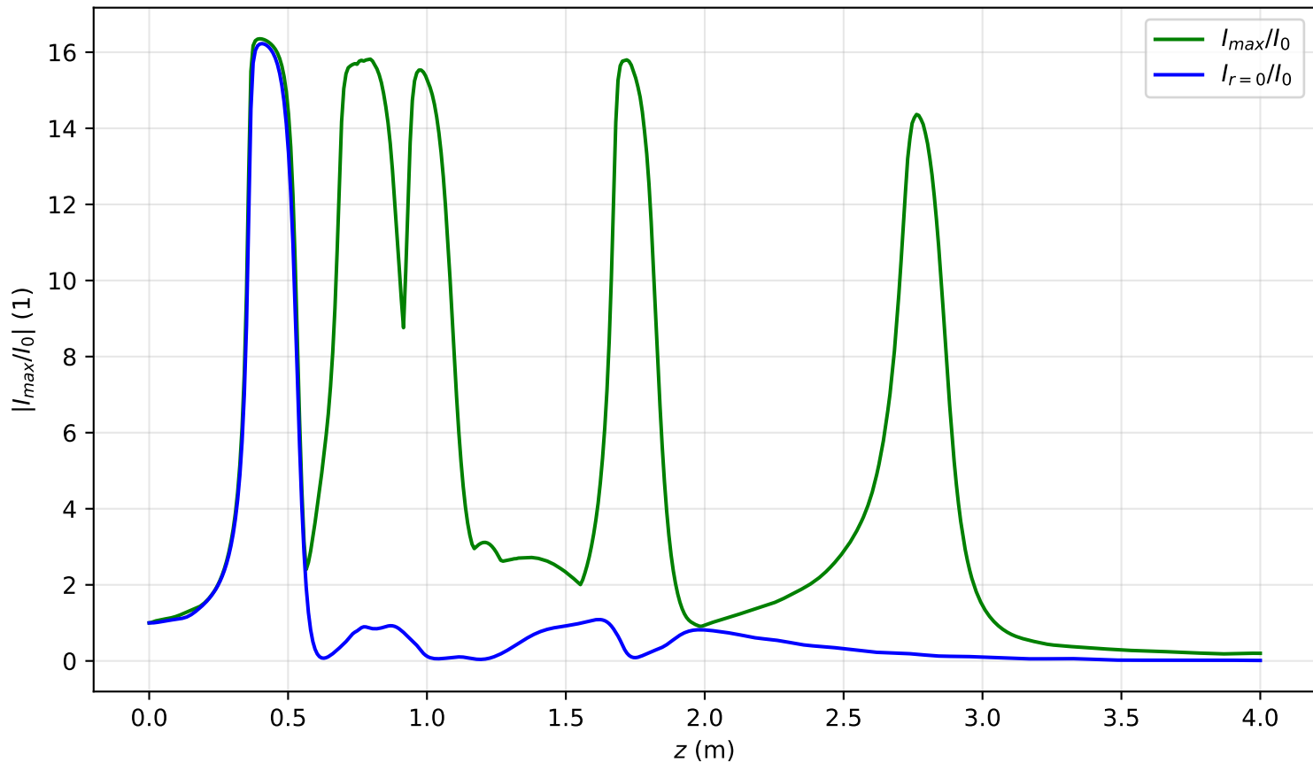
I_{max}(x = 0, y = 0, z)/I_0 , Pin=6.8Pcr, noisy input, artificial time
